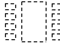
FIGURE 4. LLP Thermal Land Pad and Pin Pads
